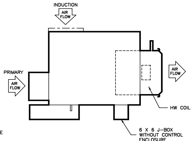
SIZES XX06, XX08, XX11 ARRANGEMENT 4
