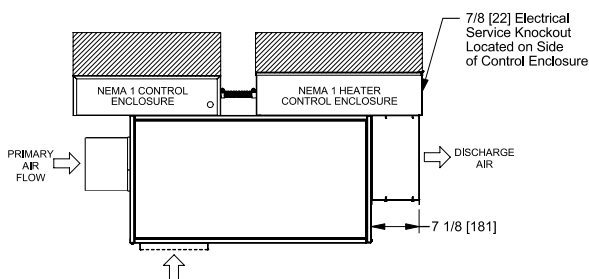
UNIT SIZES 06, 08, AND 11
