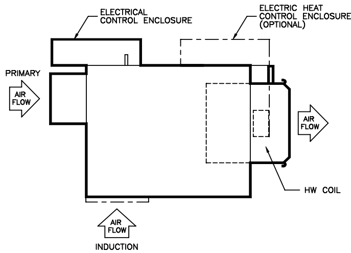
SIZES XX06, XX08, XX11 ARRANGEMENT 1
