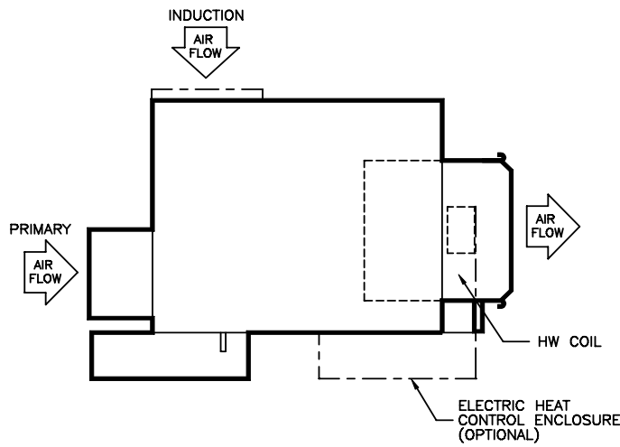
SIZES XX06, XX08, XX11 ARRANGEMENT 3
