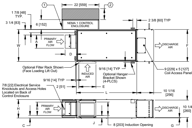
UNIT SIZES 06, 08, AND 11
