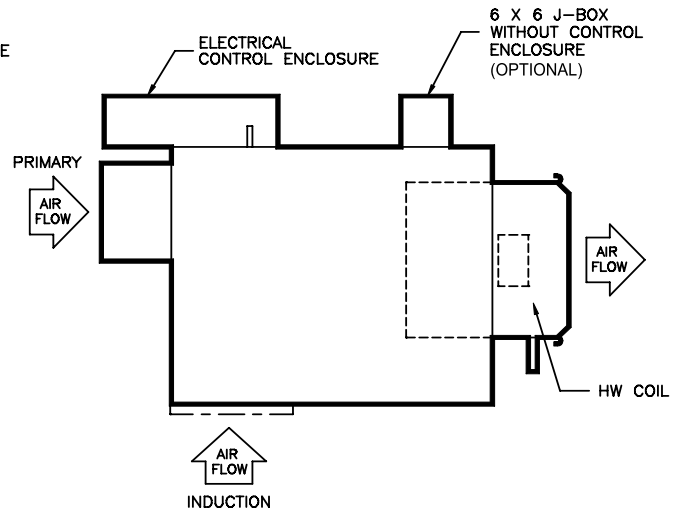
SIZES XX06, XX08, XX11 ARRANGEMENT 2
