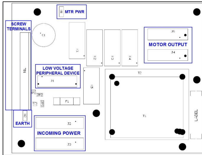
Figure 2 – Connector Layout
