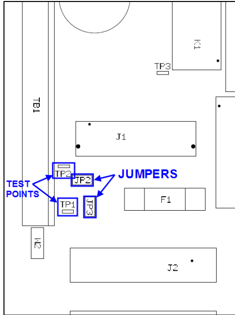
Figure F.2 - FRBii Jumpers and Test Points
